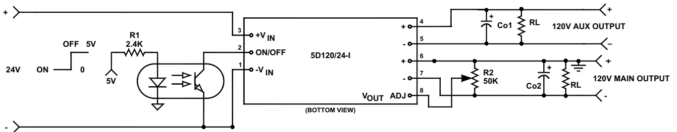
FIGURE 2. Dual connection diagram
