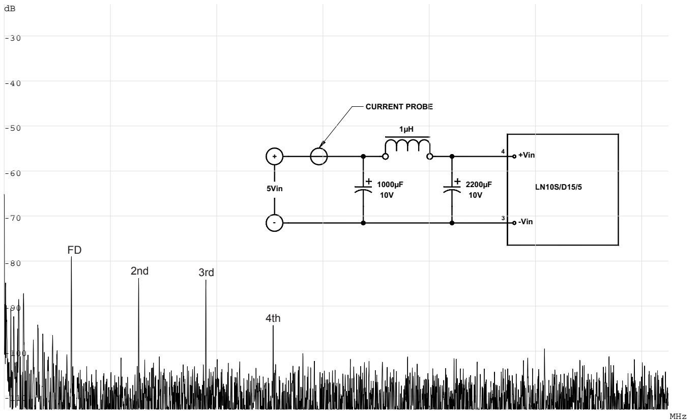
FIGURE 6. Setup and reading for reflected ripple current
