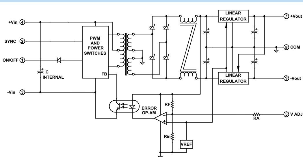
Typical Block Diagram of LN10W Dual Output Converter
