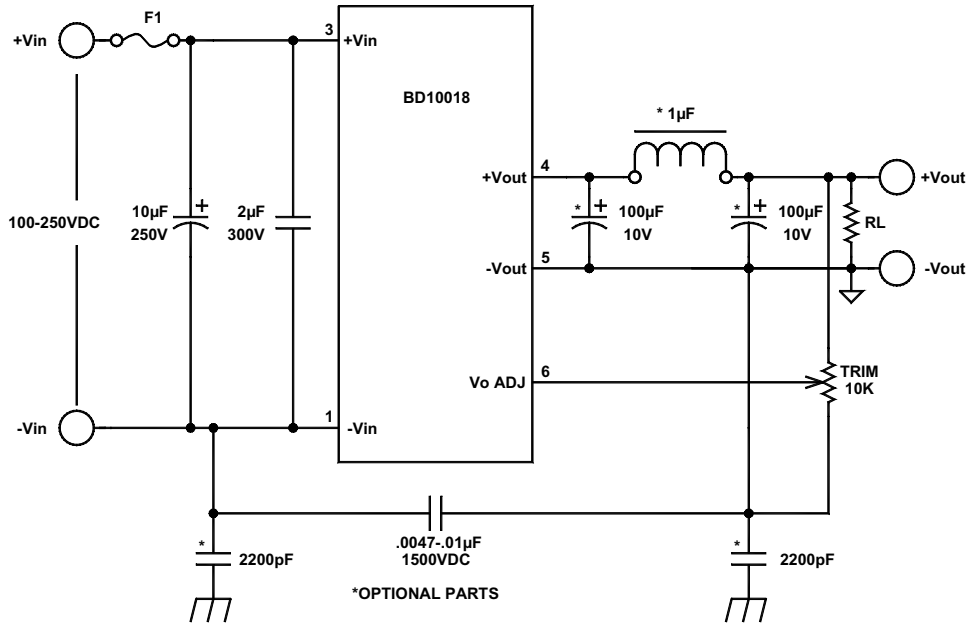
FIGURE 1. Connection diagram
