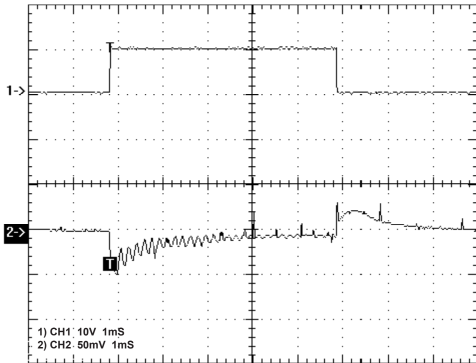
FIGURE 3. Transient response
