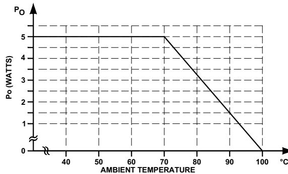
FIGURE 1. Typical derating curve
