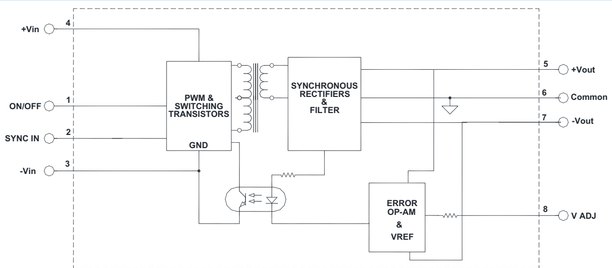
Typical Block Diagram of BHE30001 Converter
