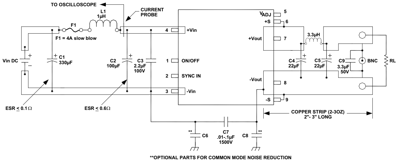
FIGURE 5. Typical setup to further reduce the output ripple for the EBL30002.
