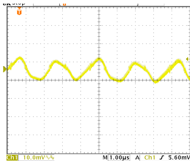
FIGURE 2. Output ripple with I_{OUT}=6A with 47\mu F@25V external output capacitors
