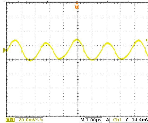
FIGURE 1. Output ripple with I_{OUT}=6A with no external output capacitors
