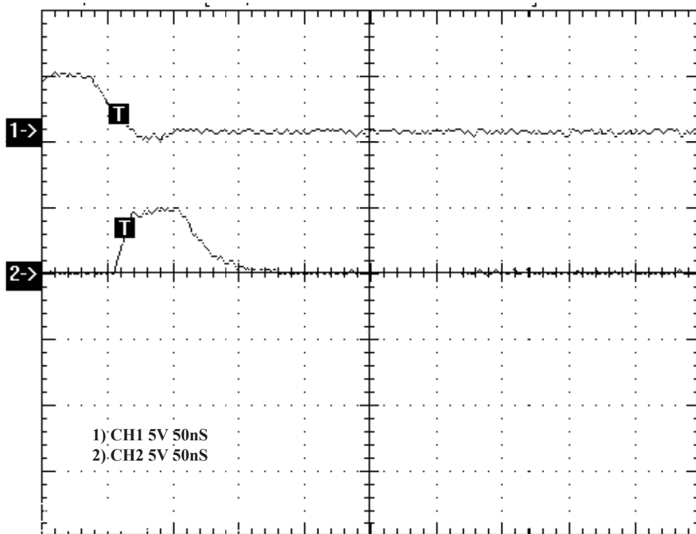
FIGURE 9. Waveforms generated from circuit in Figure 8
