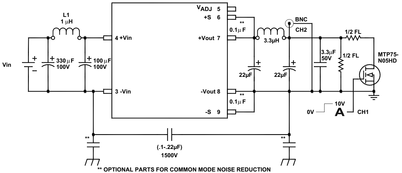
FIGURE 6. Setup for transient response measurements
