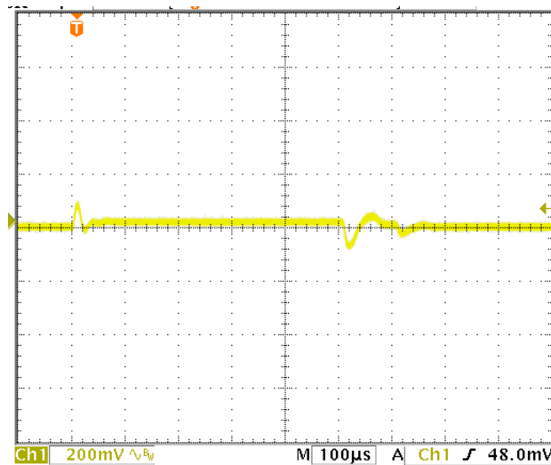
FIGURE 7. Transient response 50% full load to full load to 50% full load
