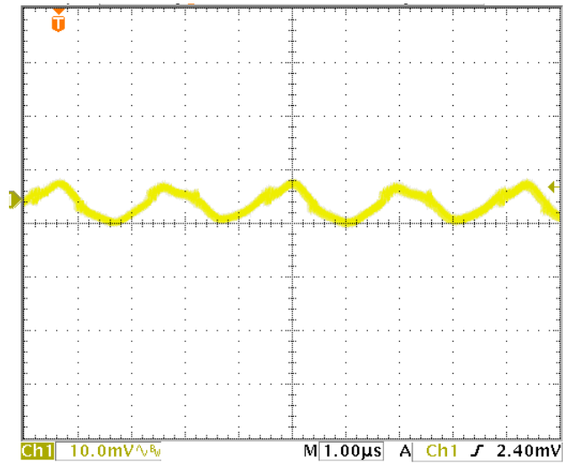
FIGURE 3. Output ripple with I_{OUT}=6A with 47\mu F@25V and 180\mu F@16V external output capacitors in parallel.
