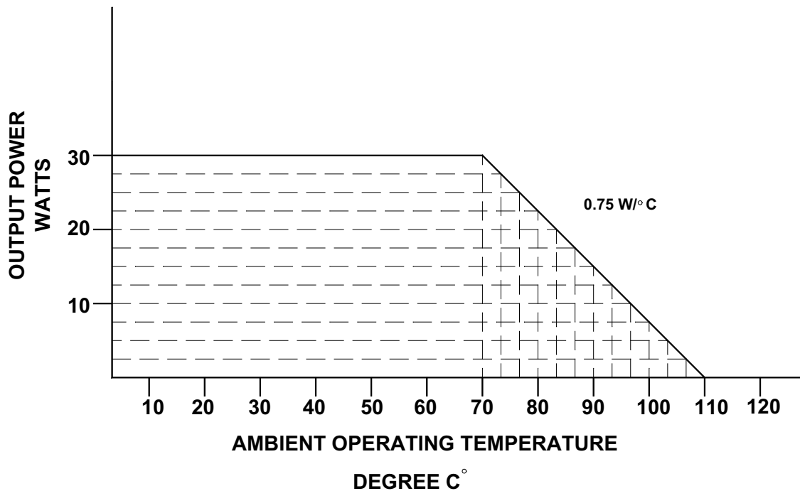
FIGURE 4. Worse case derating for the EBL30002 series
