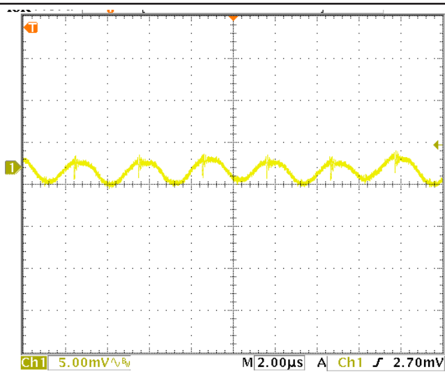
FIGURE 2. Output ripple of Figure 3
