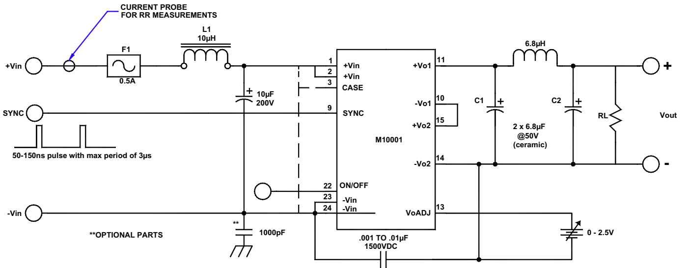
FIGURE 6. Typical connection diagram of M10001
