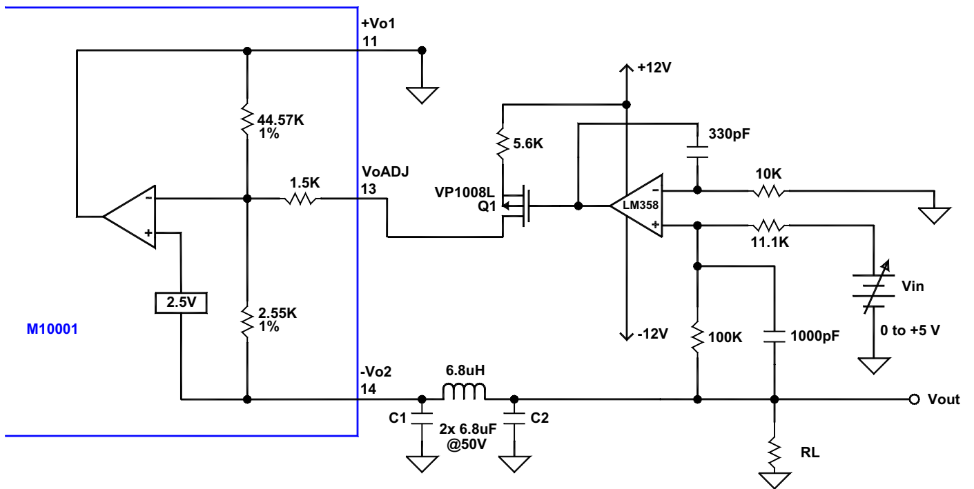
FIGURE 7. Connection diagram for M10001 for V_{IN} = 0 to 5V and V_{OUT} = 6.8 to 55V
