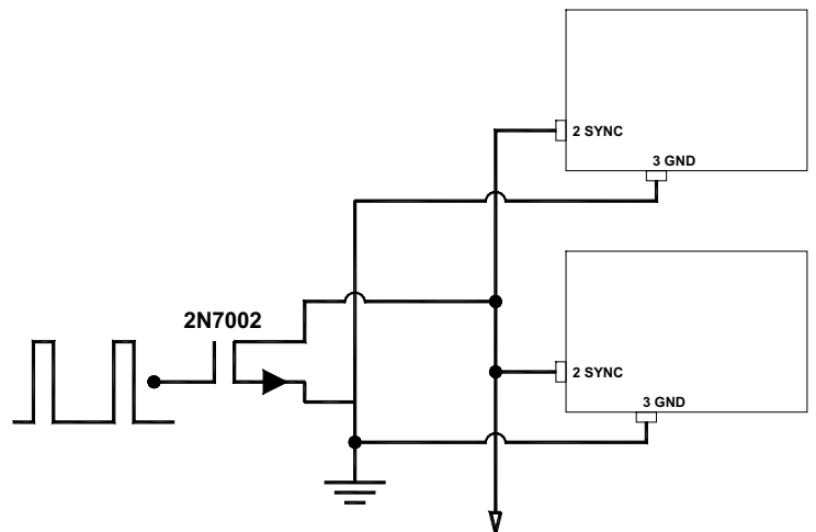
FIGURE 2. Sync of multiple devices of Q25015
