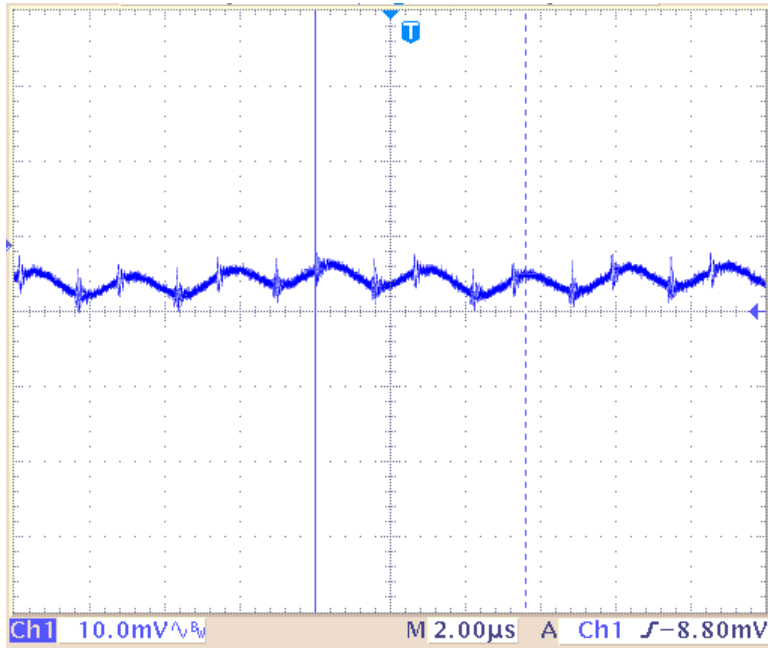
FIGURE 5. Output ripple of Q25015, V_{IN}=48V , 14V_{OUT}@I_{OUT}=1.5A , as shown in Figure 3.
