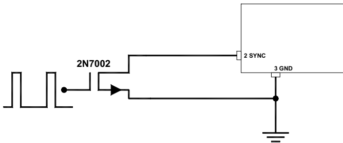
FIGURE 1. Sync from external clock for Q25015
