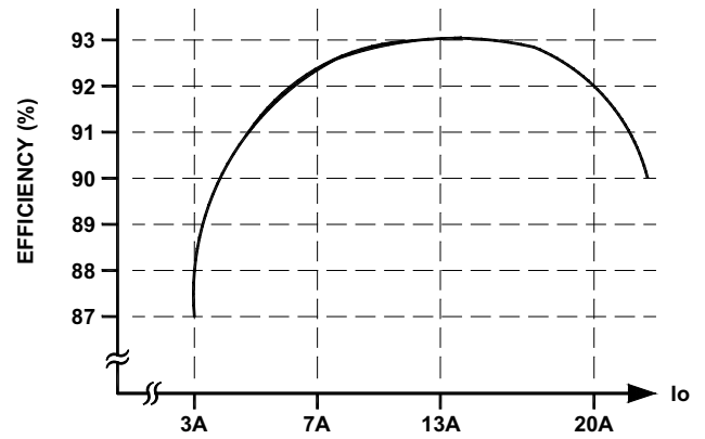
FIGURE 8B. Typical Efficiency vs. Load for 3.3V_{OUT}/48V_{IN}
