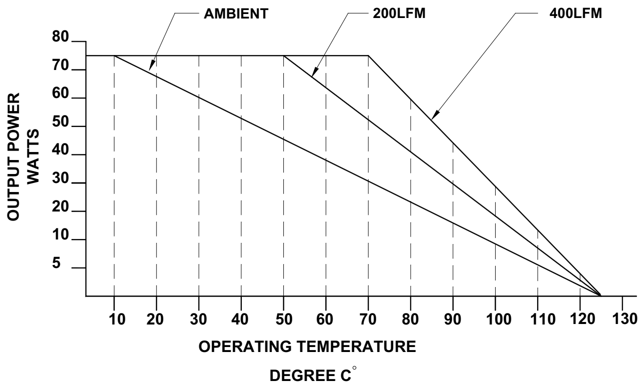
FIGURE 8. Typical derating curves for Q75007 with heat sink
