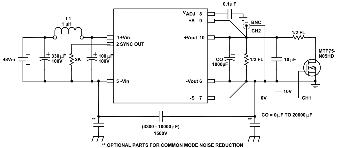
FIGURE 3A. Setup for transient response measurements
