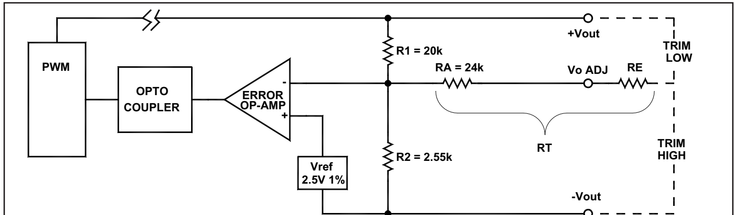
FIGURE 5. Output control circuit of 75W PowerWatt series
